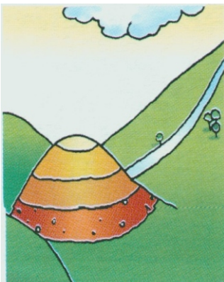
colline moreniche
