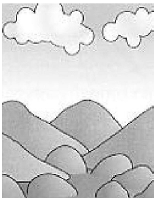
colline moreniche
